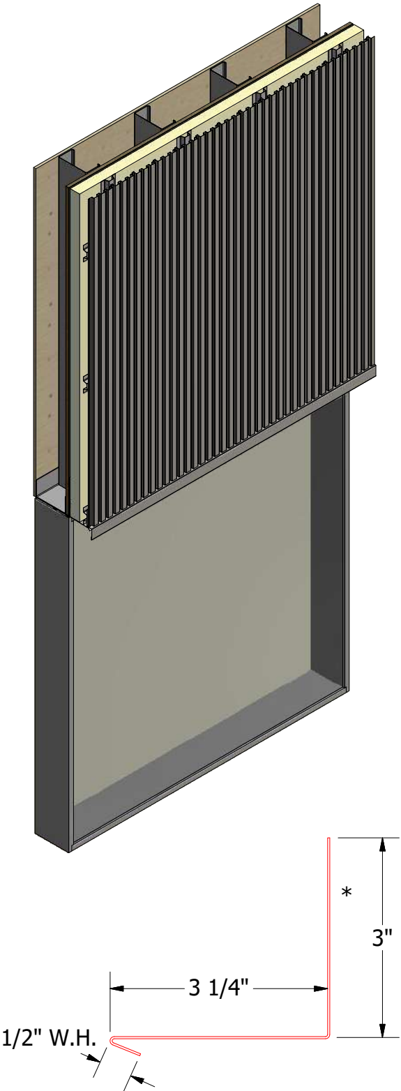
OPA683-Angle with Return
