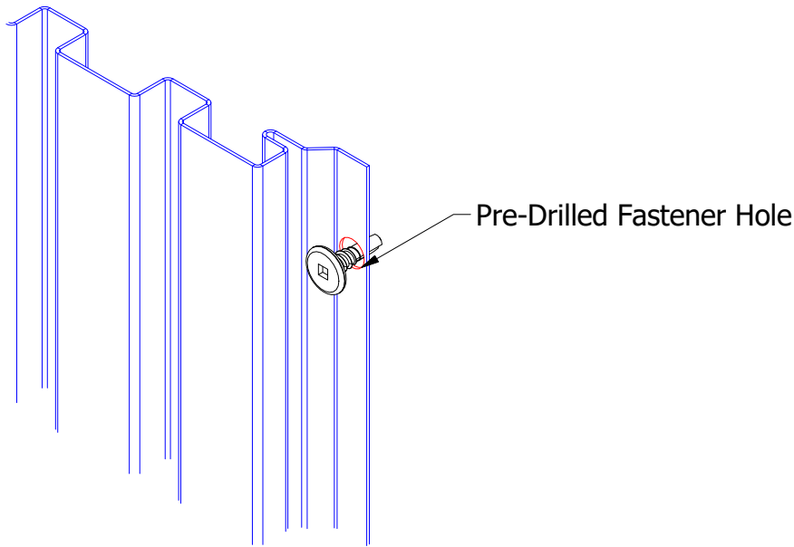
Pre-Drill Fastener Holes for Panels Greater than 20'-0" in Length
