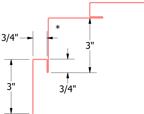
OPA601-Inside Corner Post
