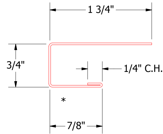
J Channel
