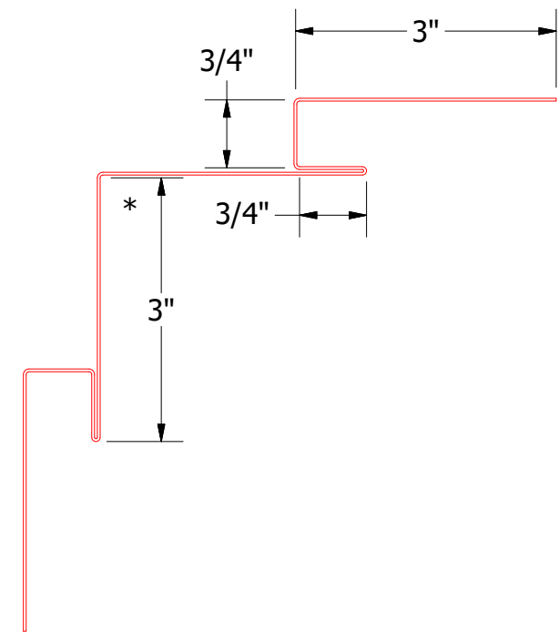
OPA601 - Inside Corner Post
