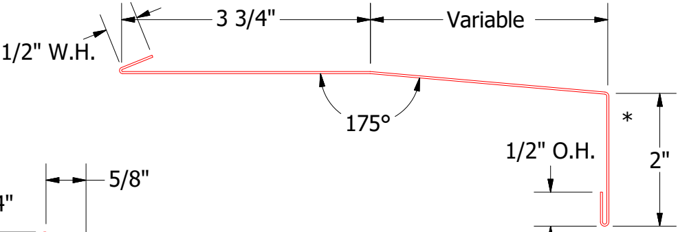
OPA670-Window Sill Trim
