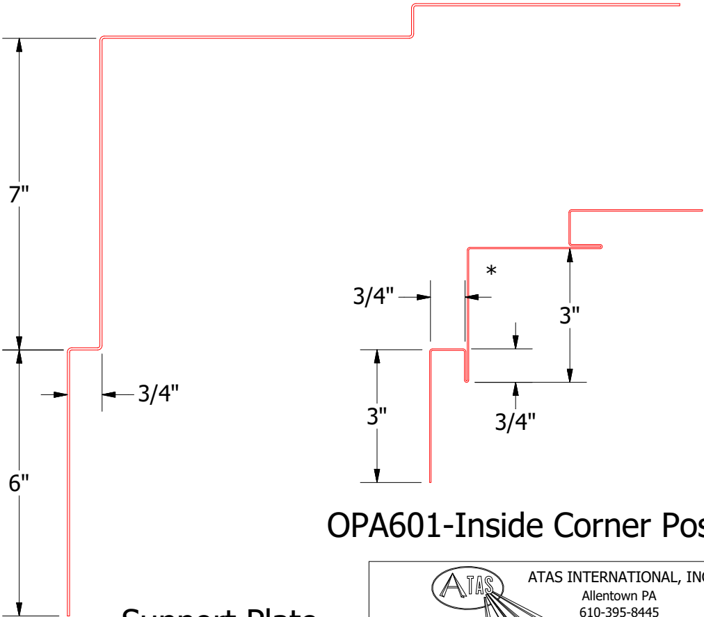
Support Plate
