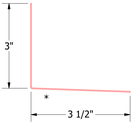
Flashing
