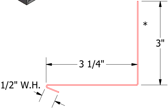
OPA683-Angle with Return
