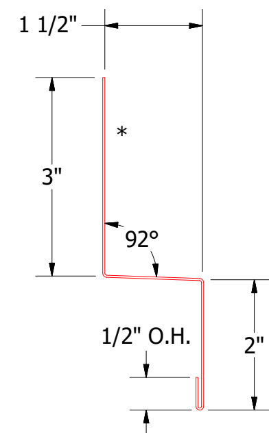
MPA550-Head Trim
