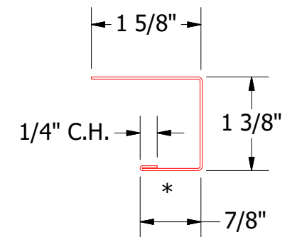
MPA138-J Channel
