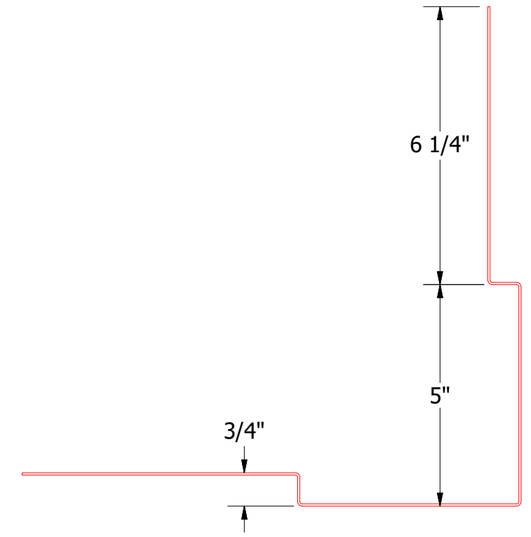
Support Plate
