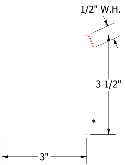
MPA683-Angle Trim with Return
