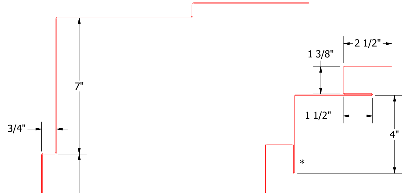
Alternate Subgirt Orientation
