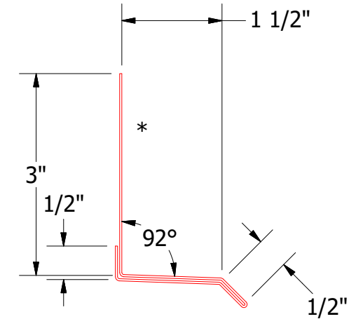
MPA661-Base Trim
