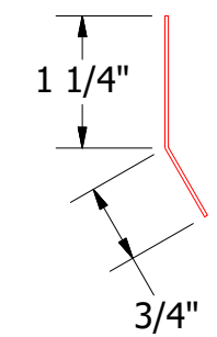
MPA103-Starter Cleat
