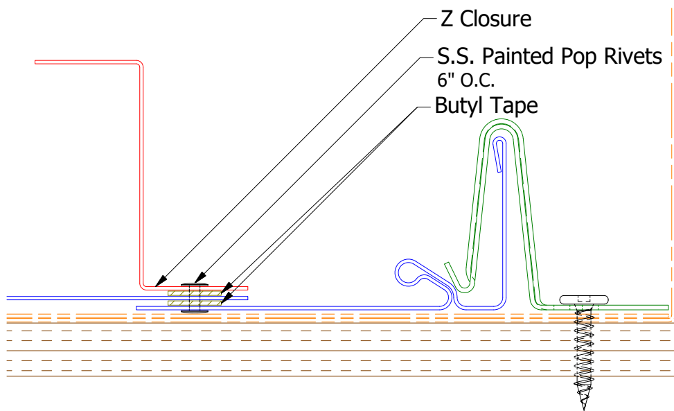
Butyl Tape Detail
