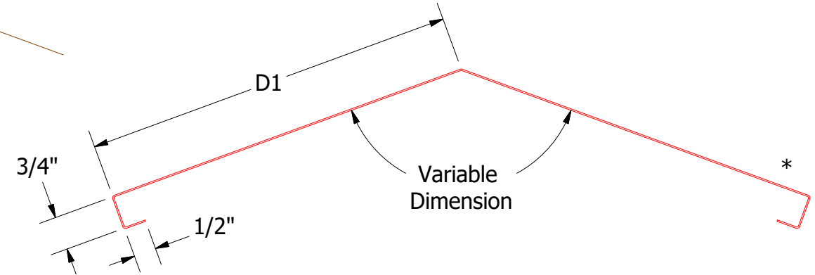
Vented Ridge Cap
