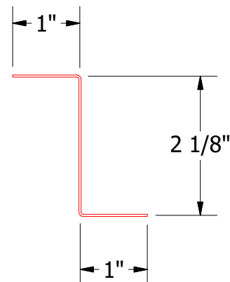
MRA910-Z Closure
