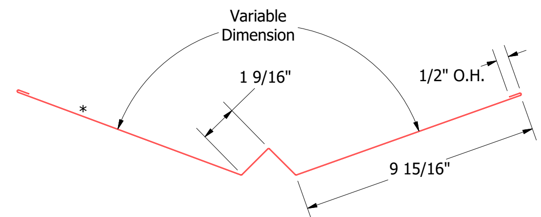
MRA800-Valley Trim
