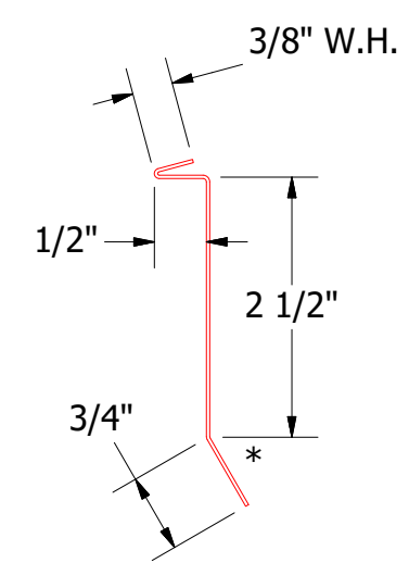
MRA980-Counterflashing
