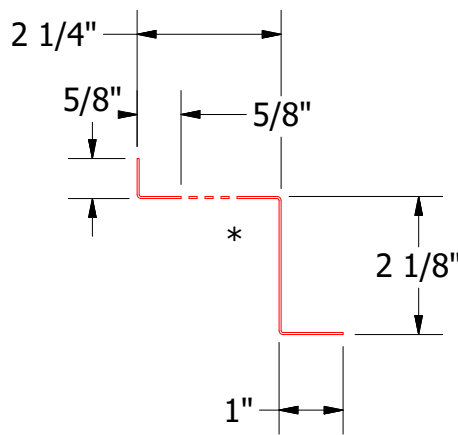
MRA911-Vented Z Closure
