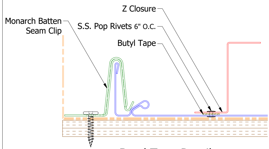
Butyl Tape Detail
