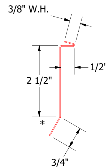
MRA980-Counterflashing
