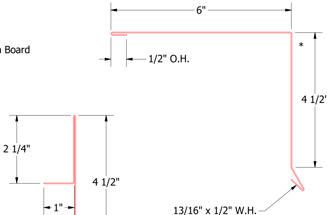
MRA210-Gable Trim
