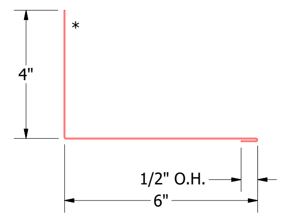
MRA410-Sidewall Trim
