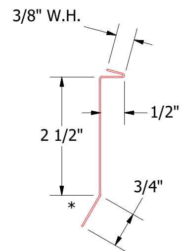
MRA980-Counterflashing
