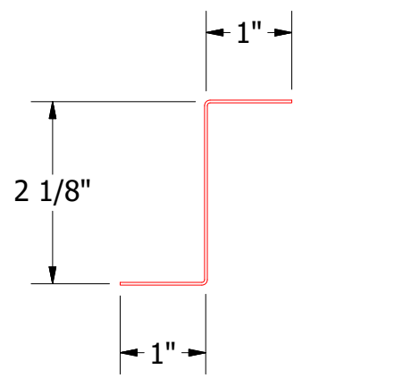
MRA910-Z Closure
