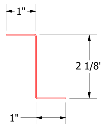
MRA910-Z Closure
