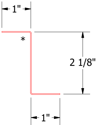
MRA910-Z Closure
