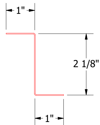
MRA910-Z Closure
