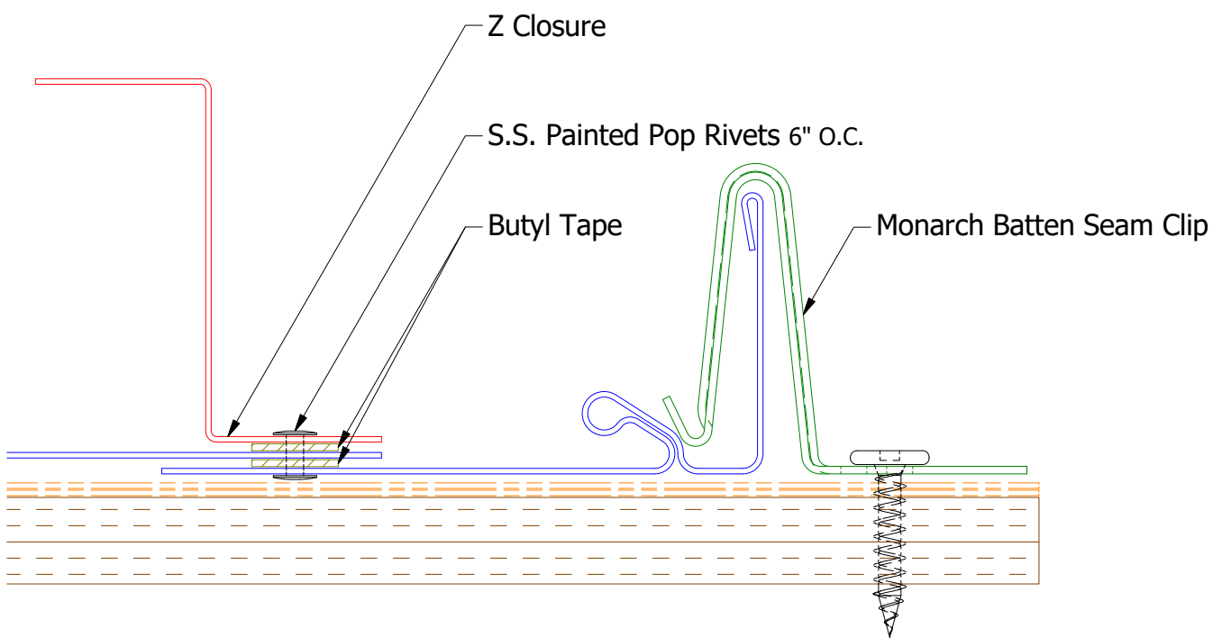
Butyl Tape Detail
