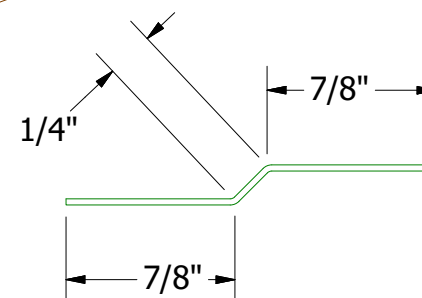
MRA975-Joggle Cleat
