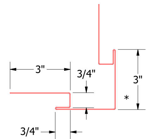
MFA602-Outside Corner Post
