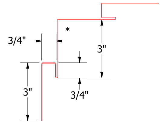
MFA601-Inside Corner Post
