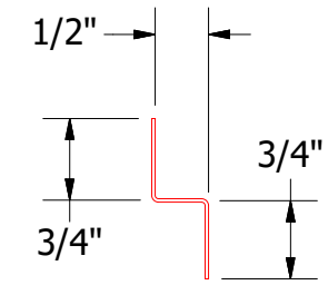
MFA681-Support Z
