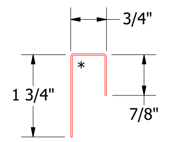
MFA270-J Closure
