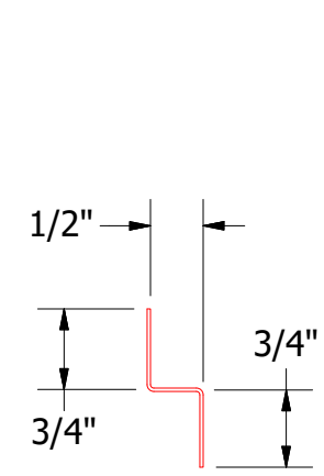
MFA681-Support Z
