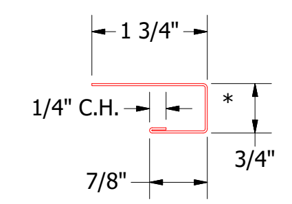
MFA034-J Channel
