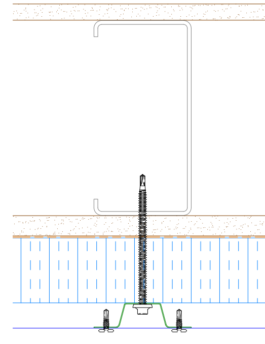
Alternate Subgirt Orientation (NTS)
