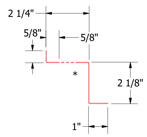
MRA911-Vented Z Closure
