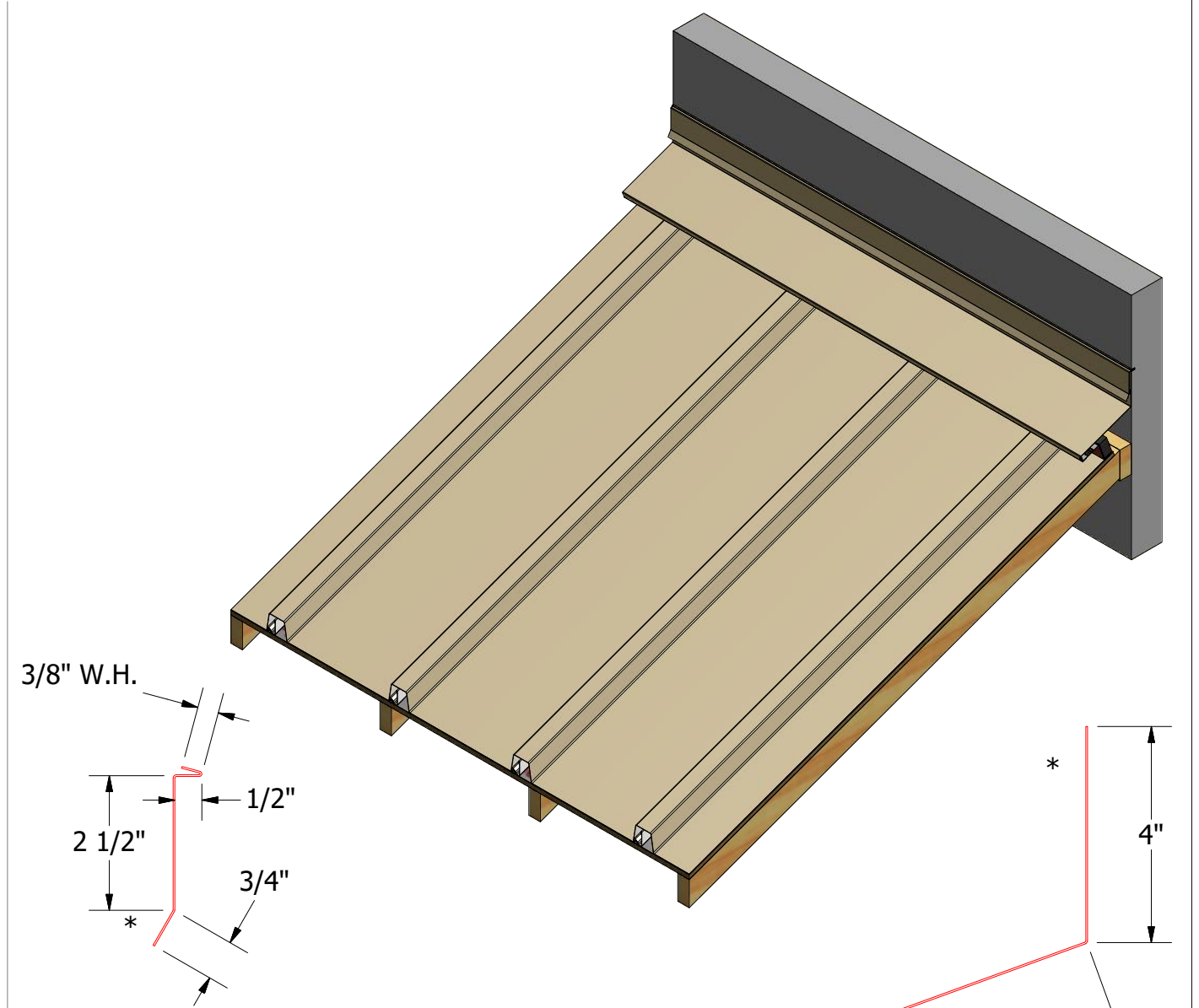
MRA980-Counterflashing
