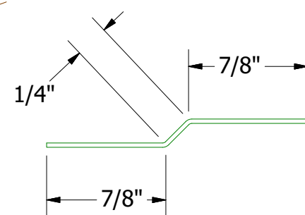
MRA975-Joggle Cleat
