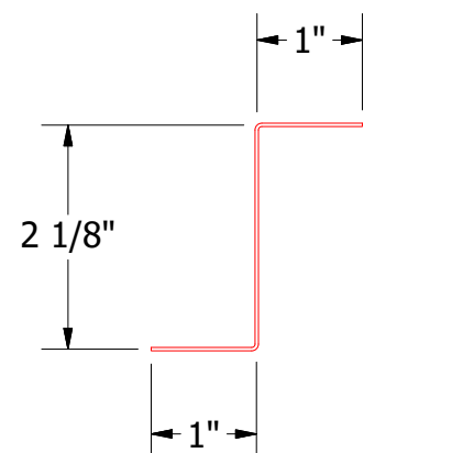
MRA910-Z Closure
