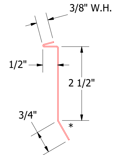
MRA980-Counterflashing
