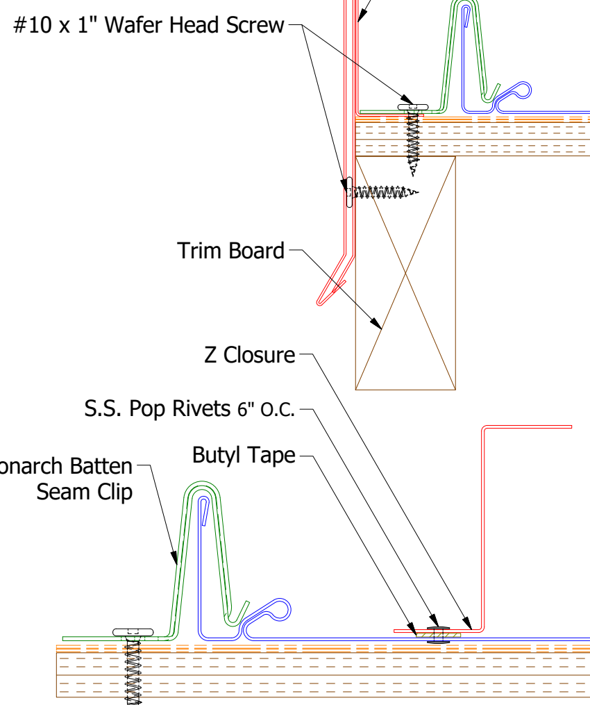
Butyl Tape Detail
