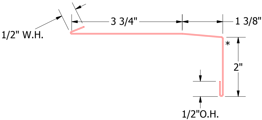
MPA670 - Window Sill Trim
