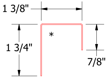
MPA270 - J Closure
