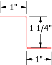
MPA681 - Support Z
