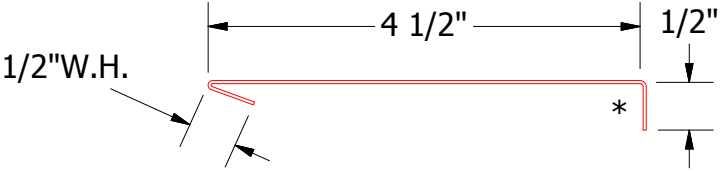
MPA690 - Head Angle Trim
