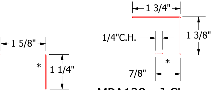
MPA138 - J Channel
