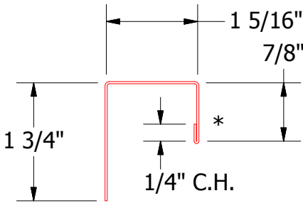
MPA134 - J Channel
