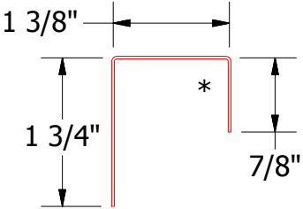
MPA270 - J Closure
