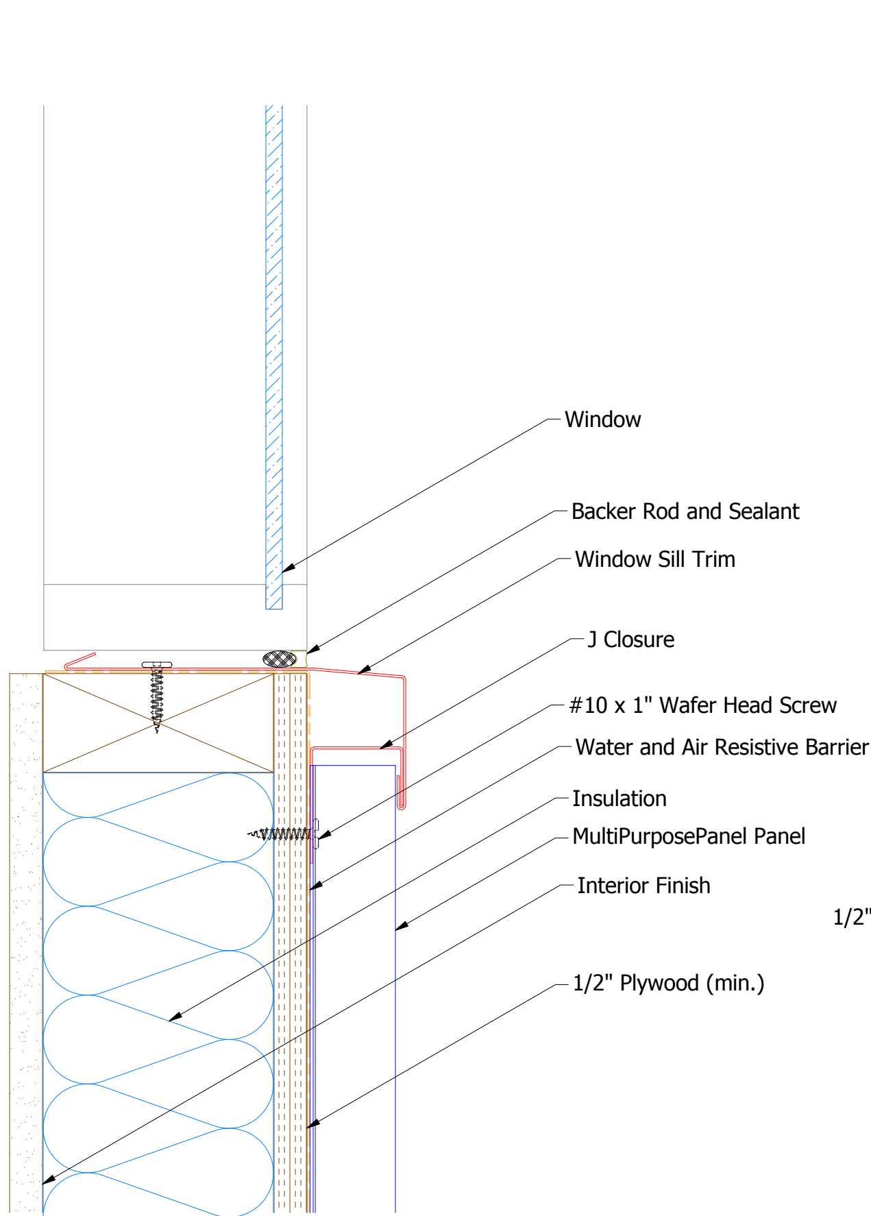
MPA670 - Window Sill Trim
