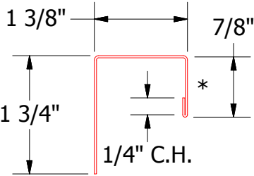
MPA138 - J Channel
