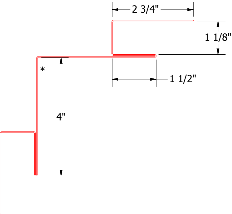
MCA601 - Inside Corner Post
