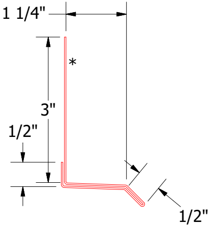
MCA661 - Base Trim
