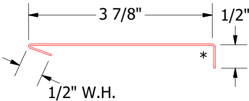
MFA690 - Head Angle Trim
