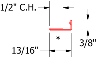
UNS078 - Snap J Cover
