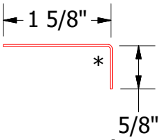
MFA680 - Angle Trim
