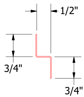
MFA681 - Support Z
