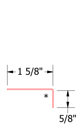
MFA680 - Angle Trim
