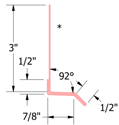
MFA661 - Base Trim
