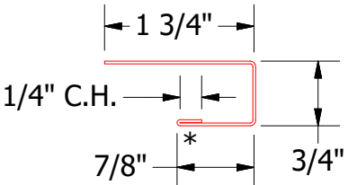
MFA034 - J Channel
