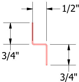
MFA681 - Support Z
