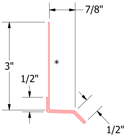
MFA661 - Base Trim
