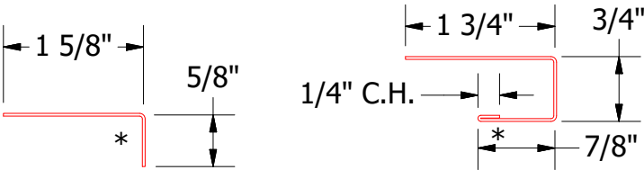
MFA680 - Angle Trim MFA034 - J Channel
