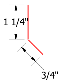
MFA995 - Starter Cleat
