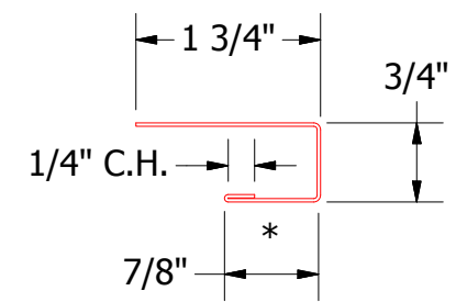
MFA034 - J Channel
