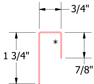
MFA270 - J Closure
