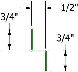
MFA681 - Support Z
