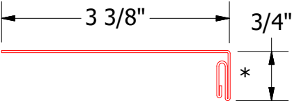
MFA039 - Snap J Base
