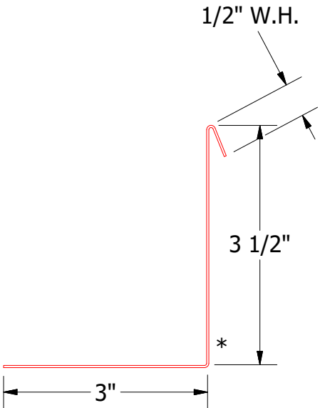
MFA683 - Angle Trim With Return
