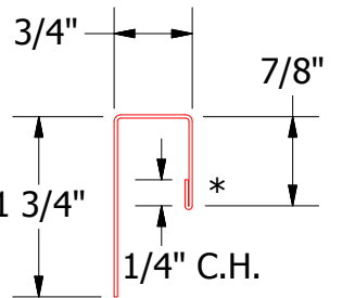
MFA034 - J Channel
