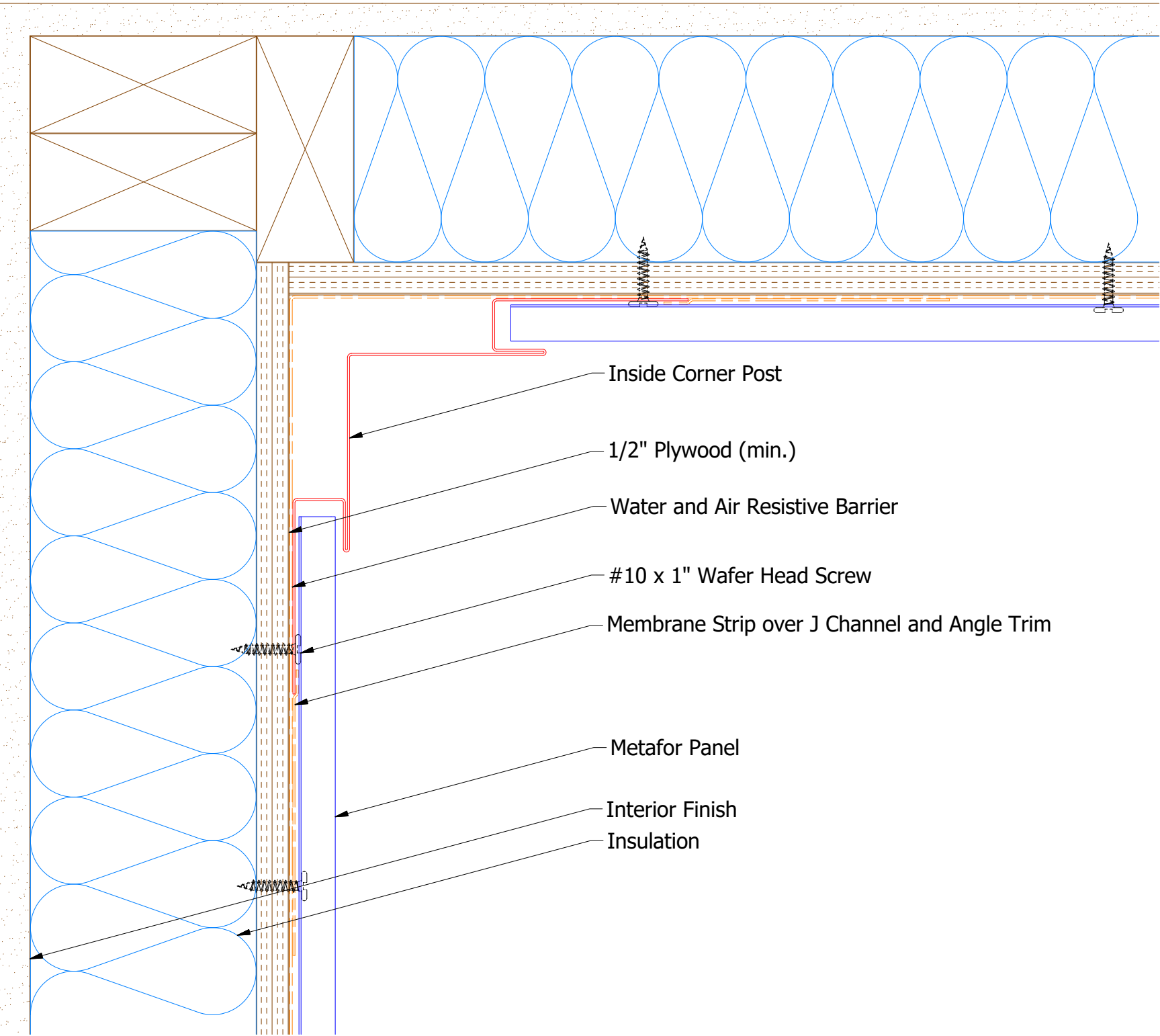
MFA601 - Inside Corner Post
