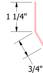
Starter Cleat
