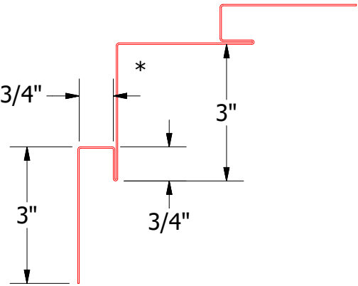
BGA601-Inside Corner Post
