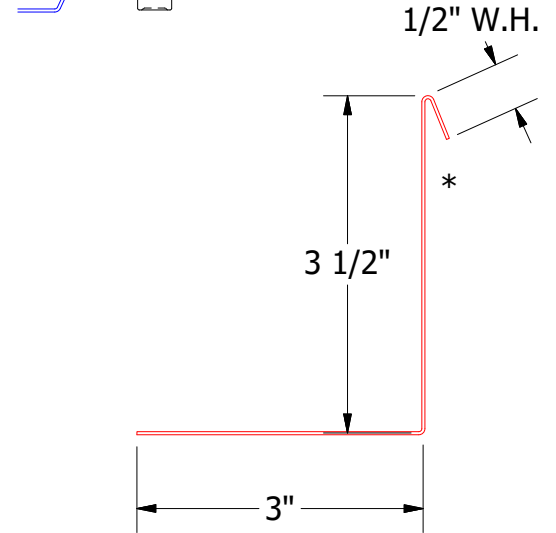
BGA683-Angle with Return
