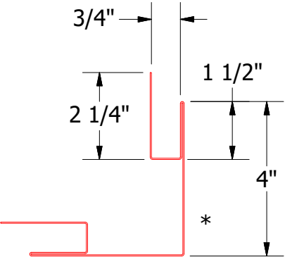
BGA602-Outside Corner Post
