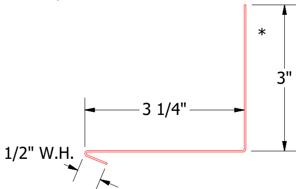
BGA683-Angle with Return
