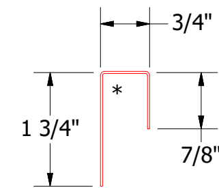
BGA270-J Closure
