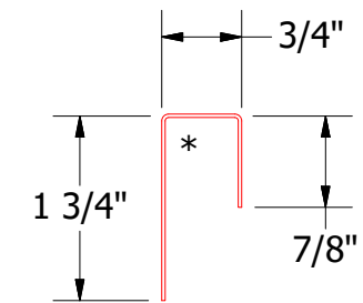
BGA270-J Closure
