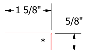
BGA680-Angle Trim
