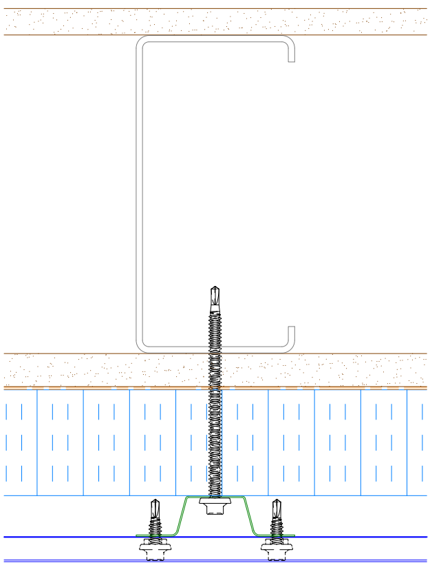
Alternate Subgirt Orientation
