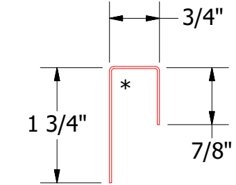
BGA270-J Closure
