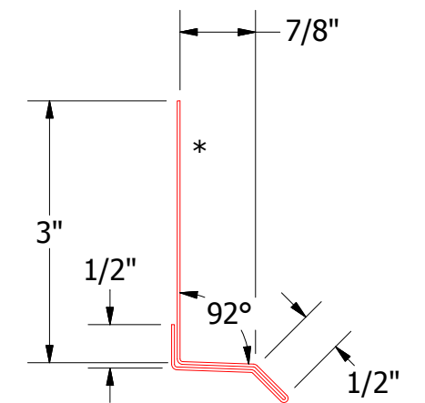
BGA661-Base Trim
