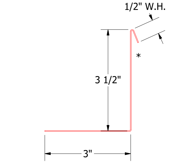
BGA683-Angle with Return
