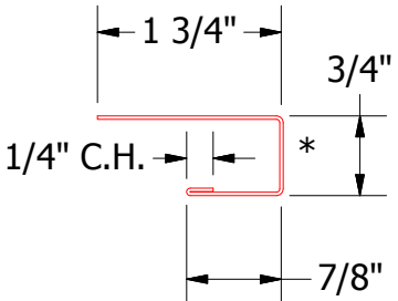
BGA034-J Channel
