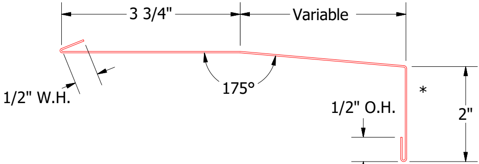
BGA673-Window Sill Trim
