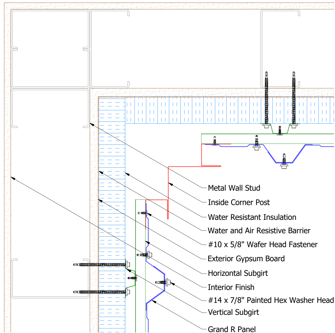
Alternative Subgirt Orientation
