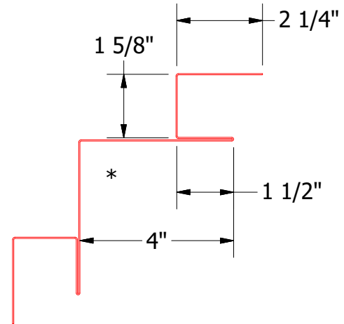
BWA601 - Inside Corner Post
