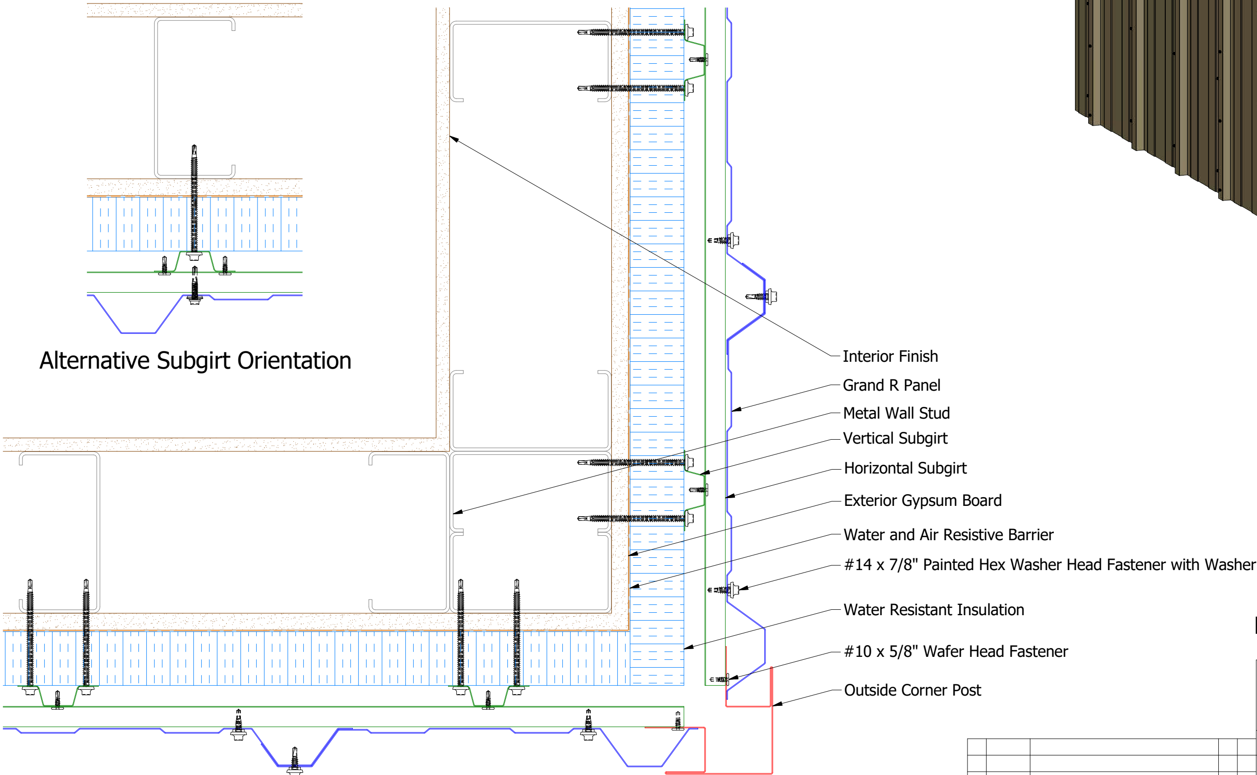
BWA602 - Outside Corner
