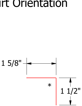
BWA160 - Angle Trim
