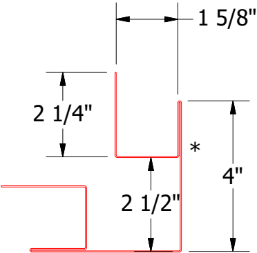
BWA602 - Outside Corner
