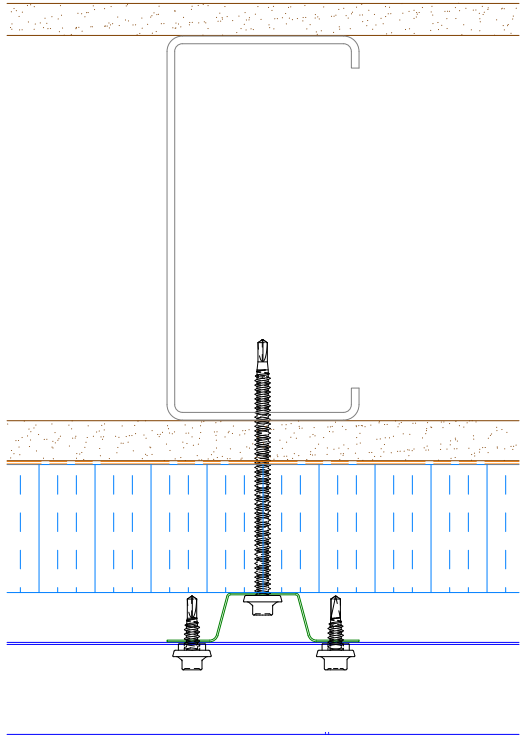
Alternative Subgirt Orientation (NTS)
