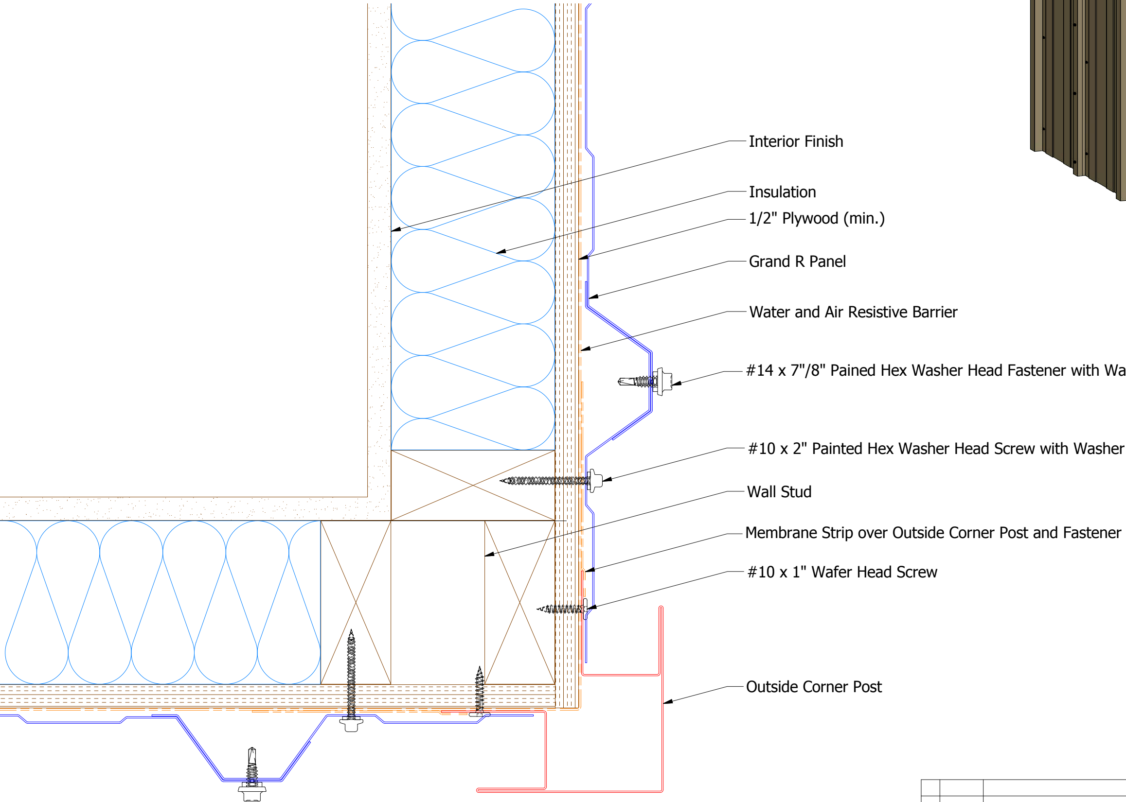
BWA602 - Outside Corner Post
