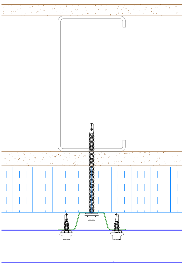
Alternative Subgirt Orientation
