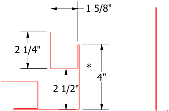
BWA602 - Outside Corner
