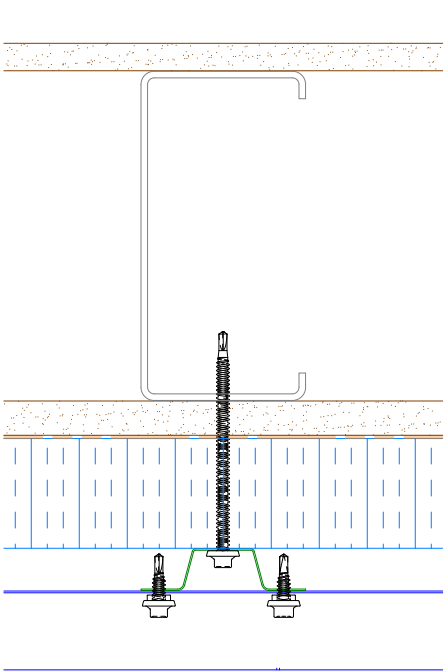
Alternative Subgirt Orientation
