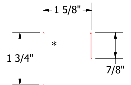
BWA270 - J Closure
