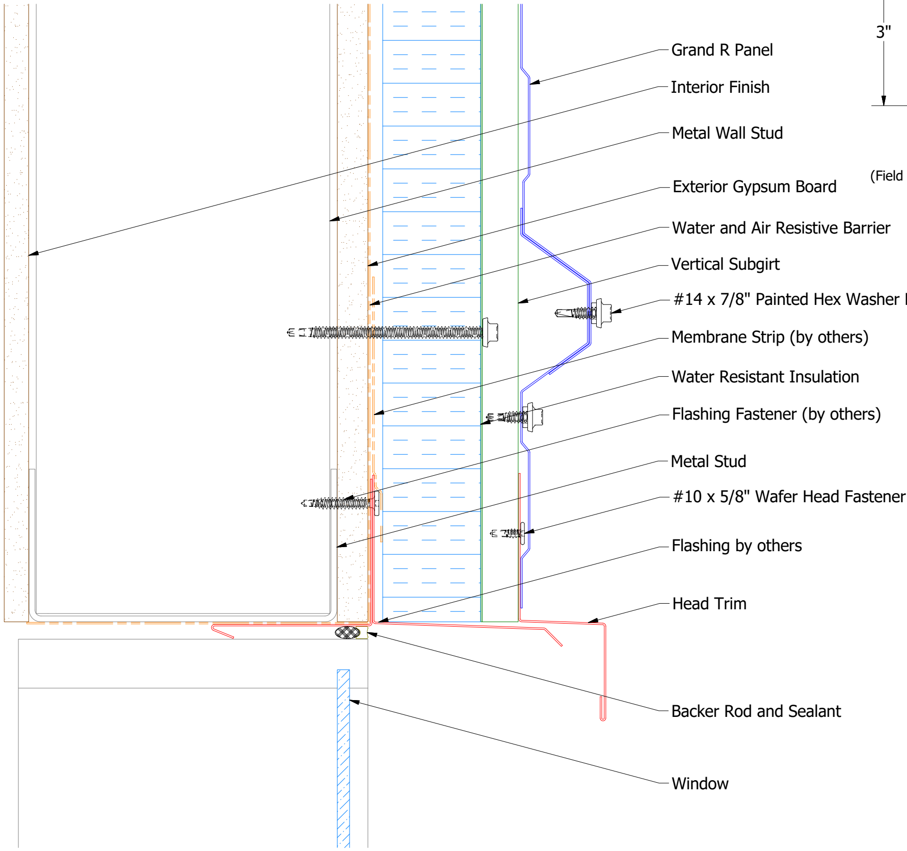
BWA550 - Head Trim
