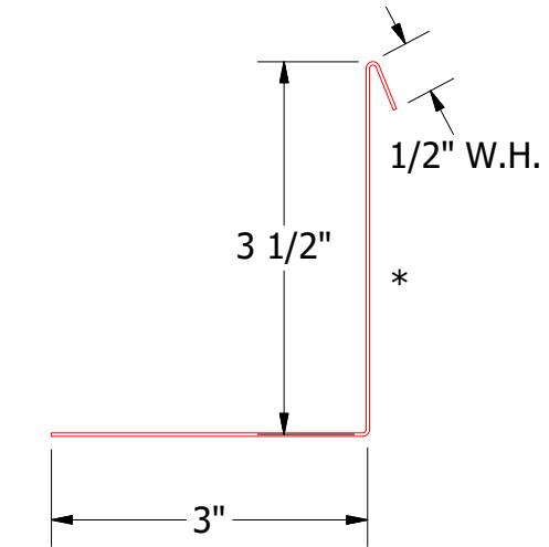
BWA683 - Angle with Return
