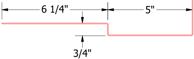
Support Plate
