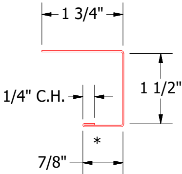
BWA158 - J Channel
