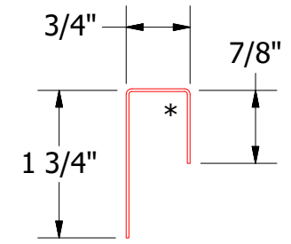
BGA270-J Closure
