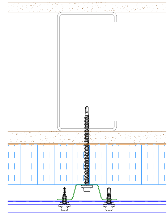
Alternate Subgirt Orientation (NTS)
