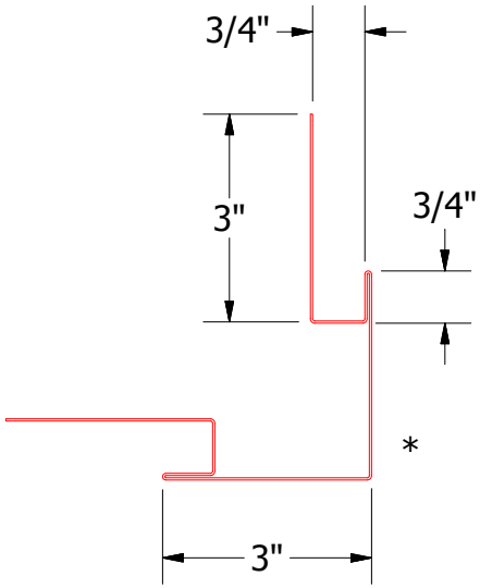
BGA602-Outside Corner Post
