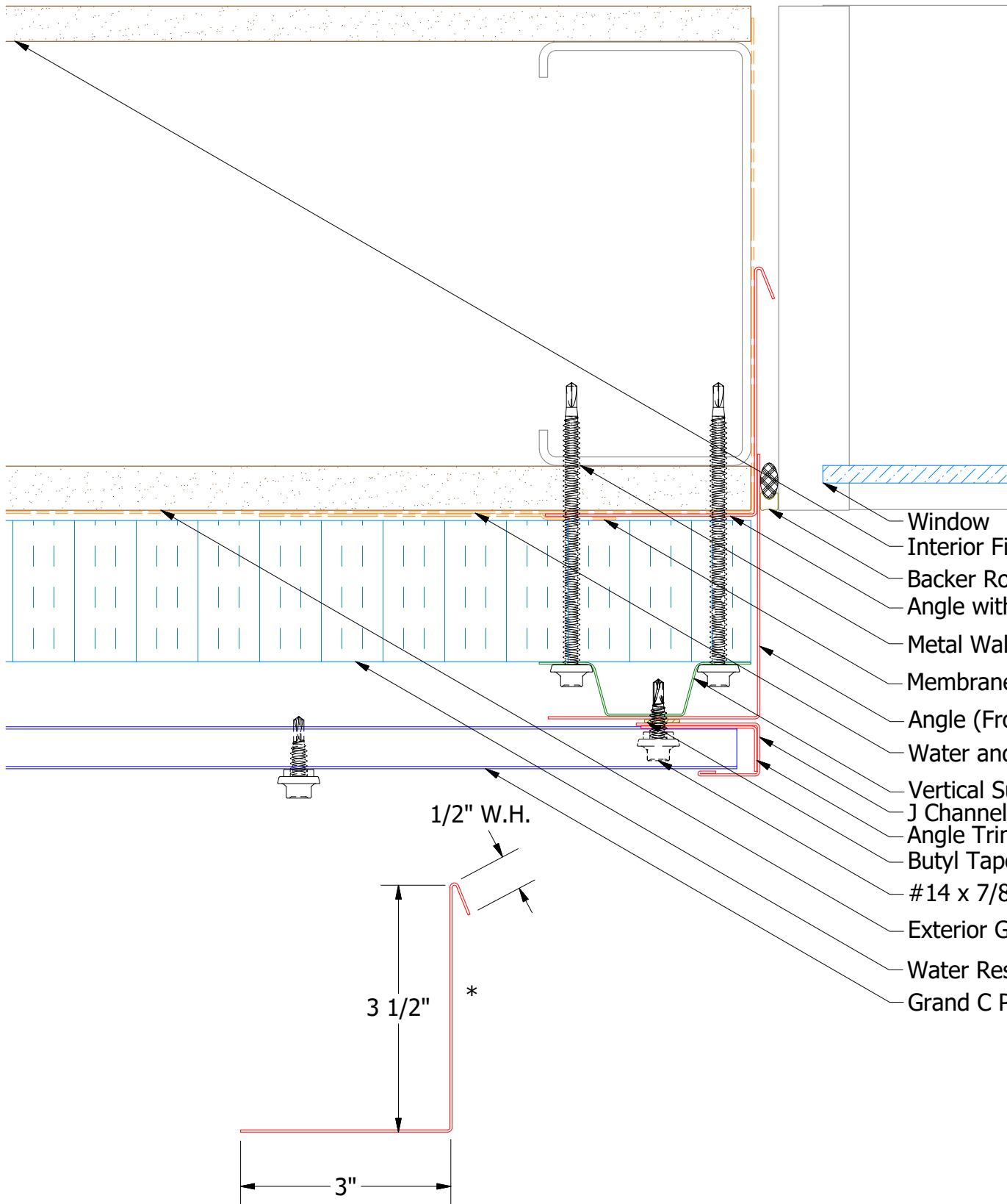
BGA683-Angle with Return
