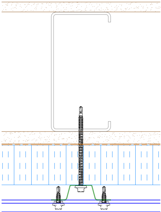
Alternate Subgirt Orientation (NTS)
