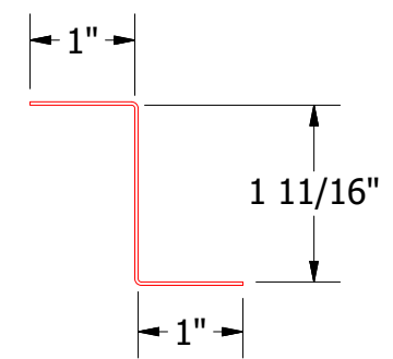
MDA910-Z Closure
