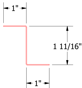
MDA910-Z Closure
