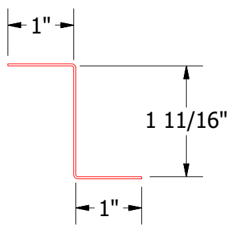
MDA910-Z Closure
