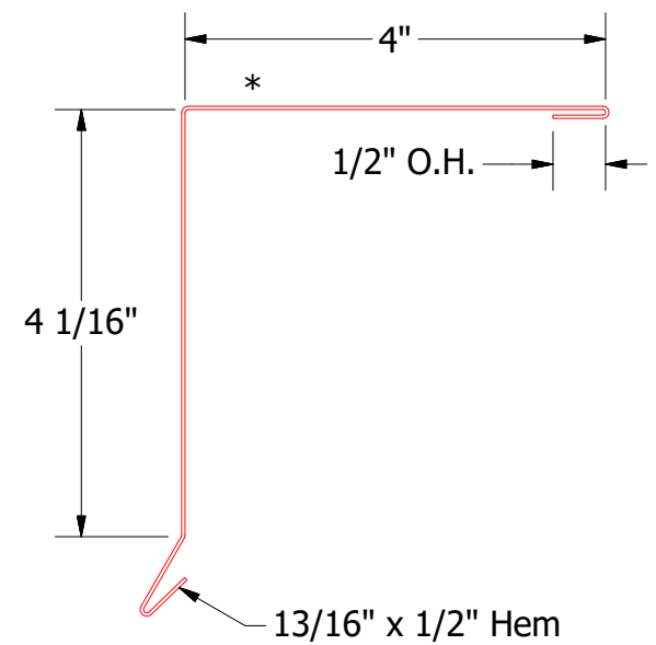
MDA210-Gable Trim Cap
