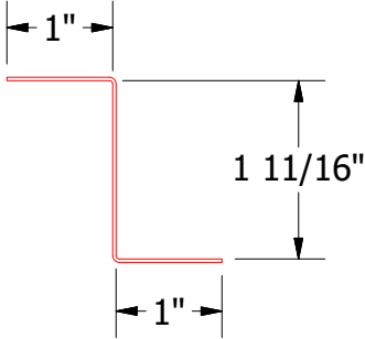
MDA910-Z Closure
