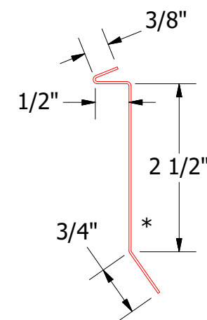
MDA980 - Counterflashing
