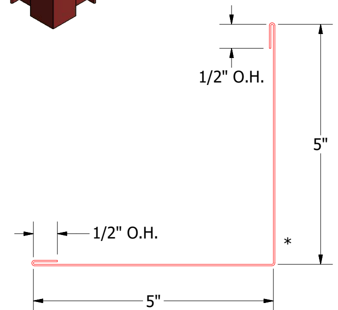
MDA610 - Outside Corner Cap
