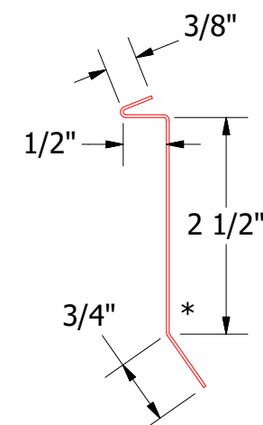
MDA980 - Counterflashing
