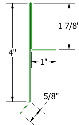
MDA211-Gable Starter Cleat
