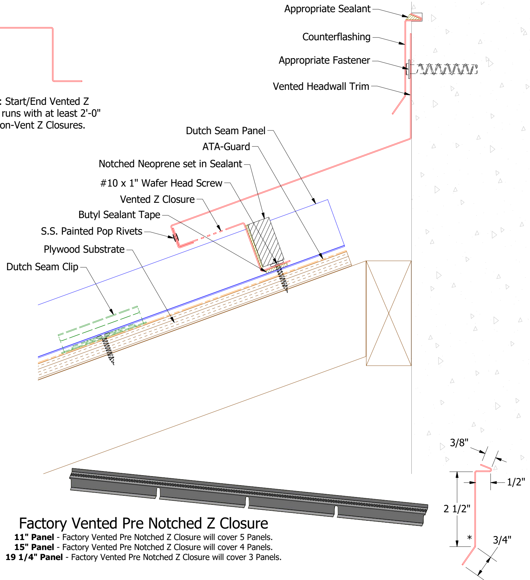
MDA980-Counterflashing
