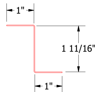
MDA910 - Z Closure
