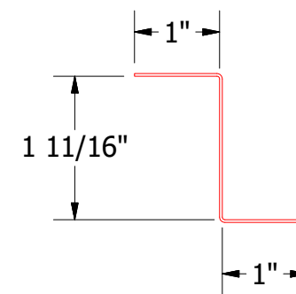
MDA910-Z Closure
