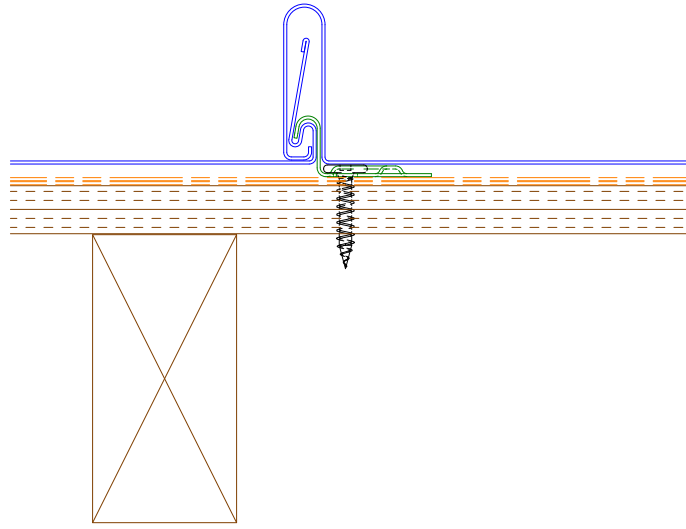
Positive Panel Interlock
