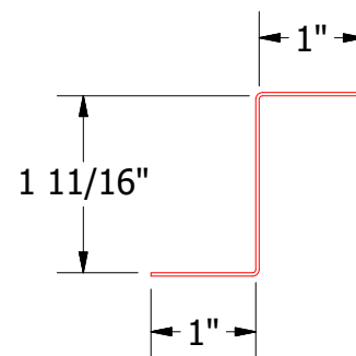
MDA910-Z Closure
