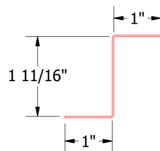
MDA910 - Z Closure
