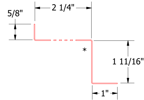
MDA911 - Vented Z Closure
