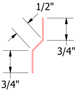
Joggle Cleat DWA975/DSA975
