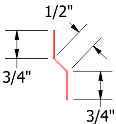
Joggle Cleat DWA975/DSA975
