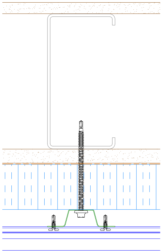
Alternative Subgirt Orientation
