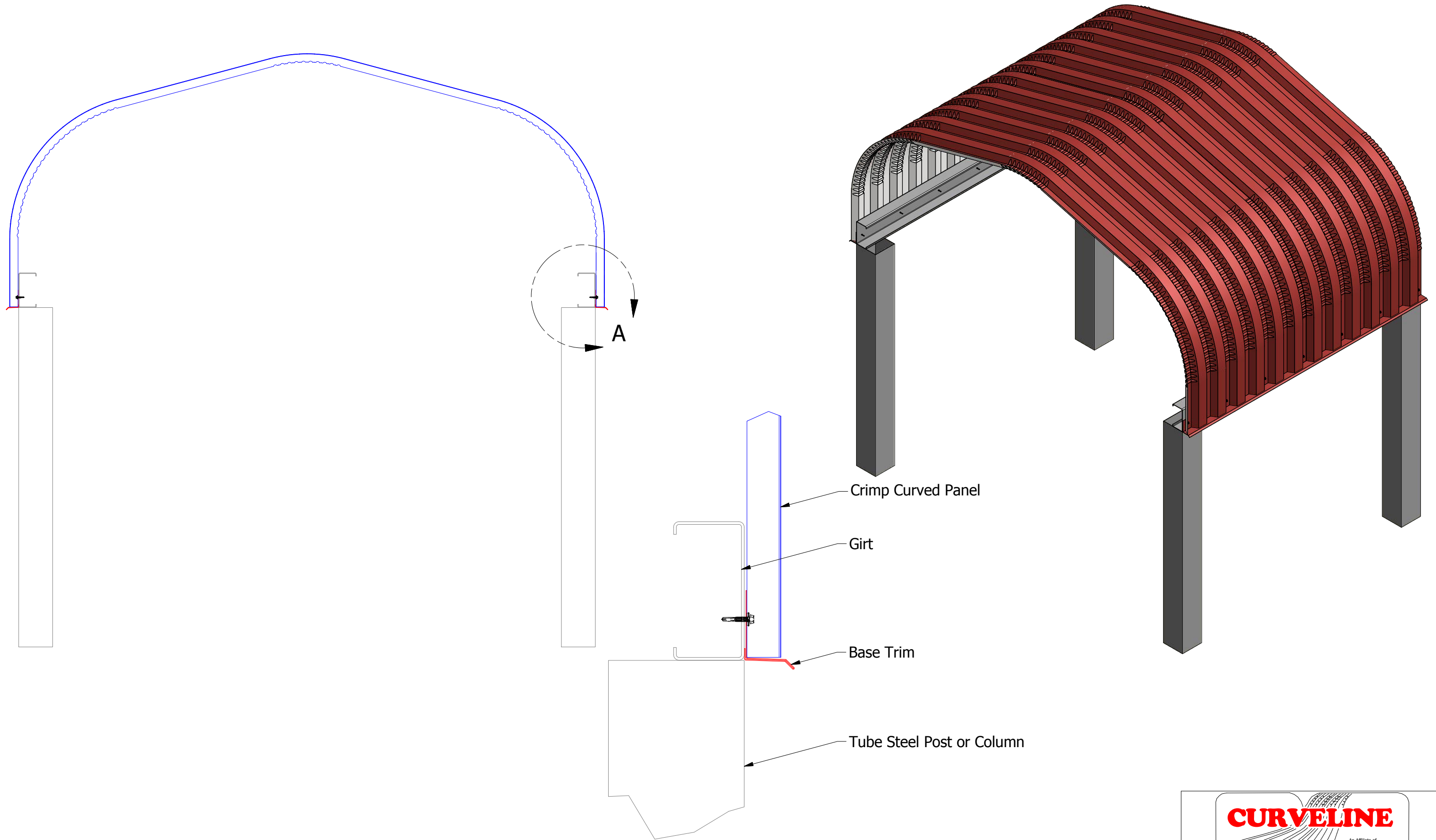
DETAIL A
