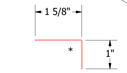
BCA680-Angle Trim
