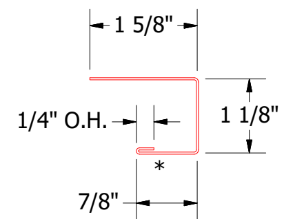
BCA118-J Channel
