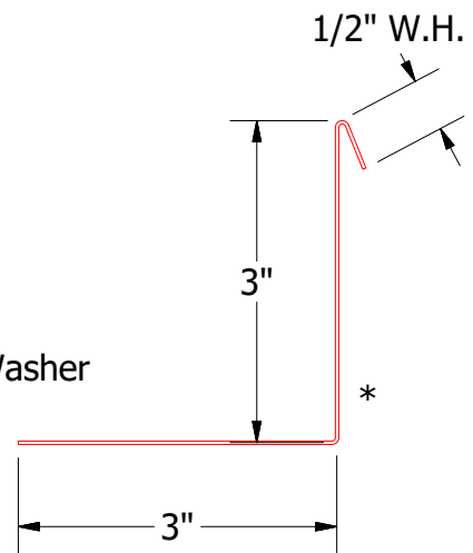
BCA683-Angle Trim with Return
