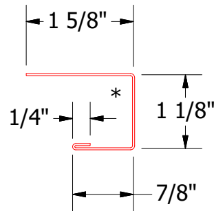
BCA118-J Channel
