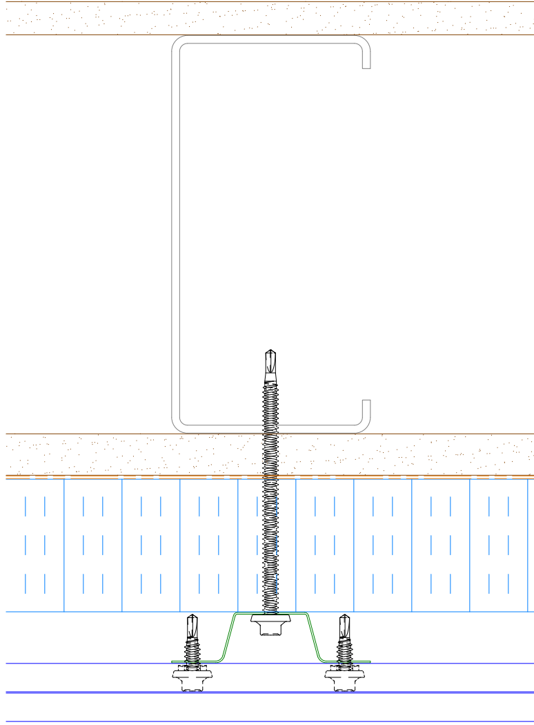
Alternative Subgirt Orientation
