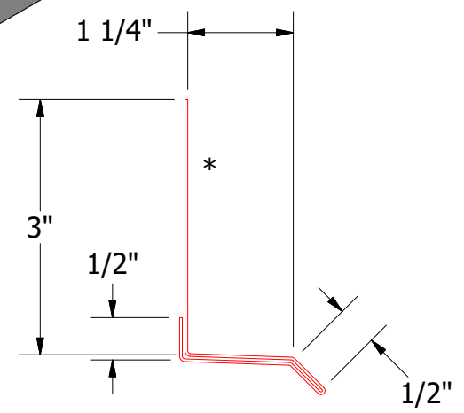
MCA661-Base Trim
