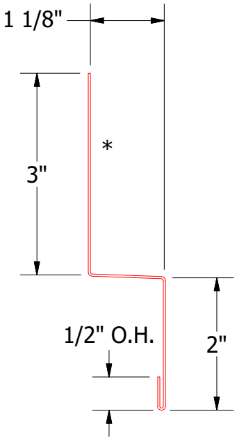
MCA550-Head Trim
