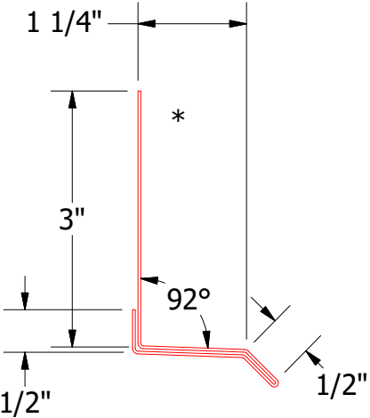
MCA661 - Base Trim
