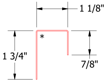
MCA270 - J Closure
