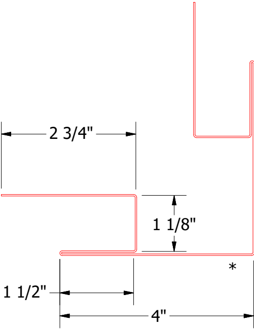
MCA602 - Outside Corner Post
