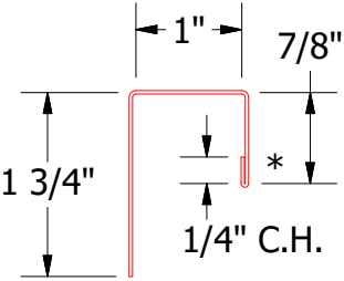
MCA118 - J Channel
