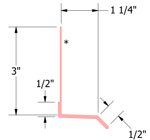
MCA661 - Base Trim
