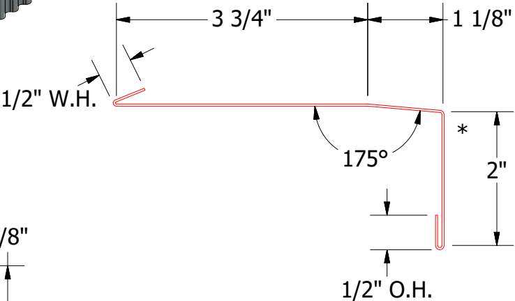
MCA670 - Window Sill Trim
