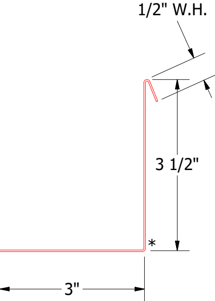
MCA683 - Angle Trim With Return
