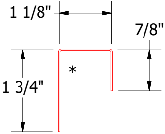
MCA270 - J Closure
