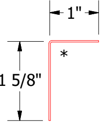
MCA680 - Angle Trim
