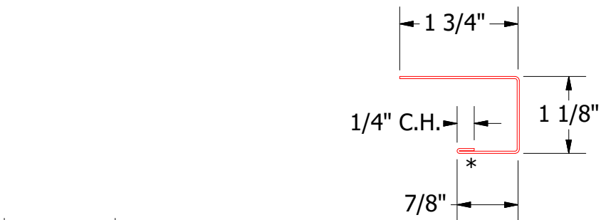
MCA118 - J Channel
