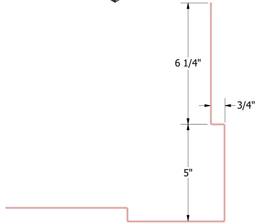
Support Plate
